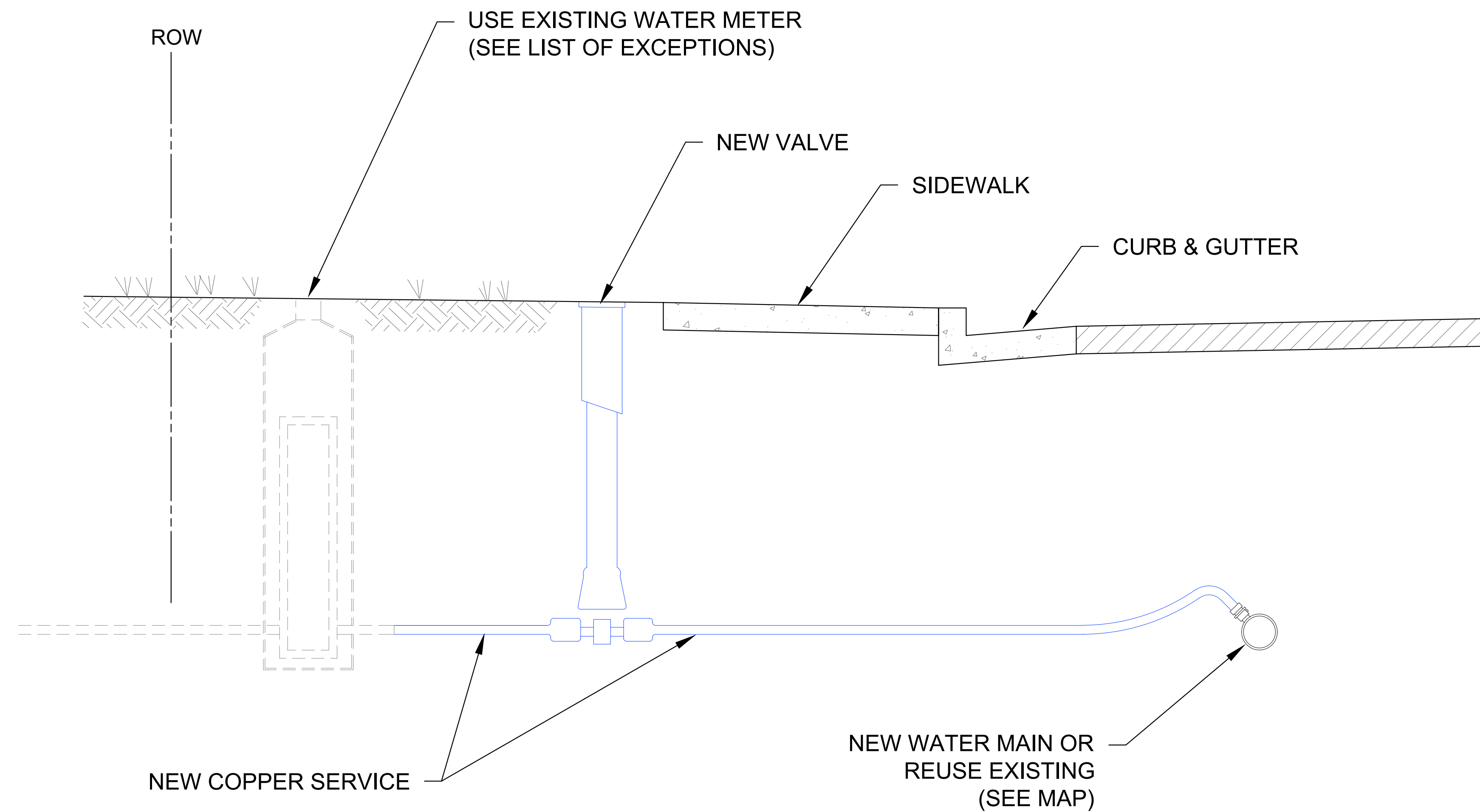
WATER SERVICE DETAIL
